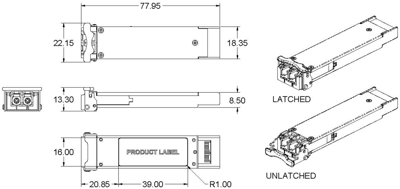
XFP Transceiver (dimensions are in mm)
